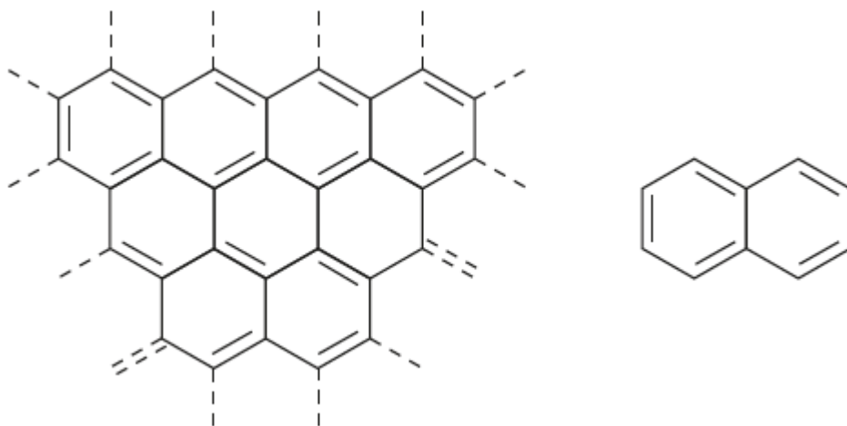
Fig. 1: Structures of graphene (left) and naphthalene (right)
