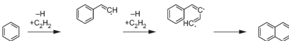
Fig. 2: The mechanism of PAH growth
